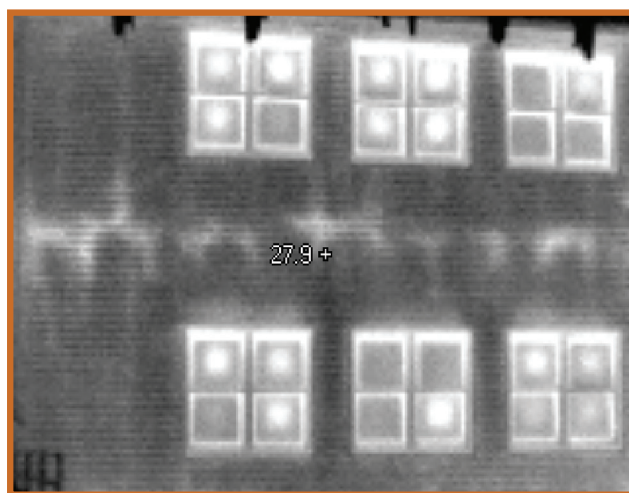
Many, but not all, infrared imaging systems in the market today comply with the minimum specifications of the new RESNET standard and, when conditions are correct, produce high quality results like this showing poorly fitted fiberglass and failing argon windows.
